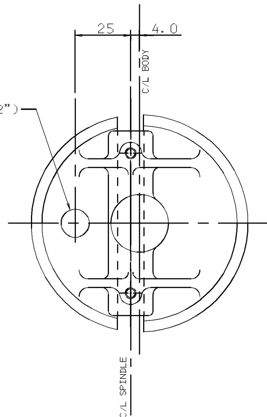
BUTTERFLY DETAIL SHOWING Ø12.7 (1/2") ORIFICE
