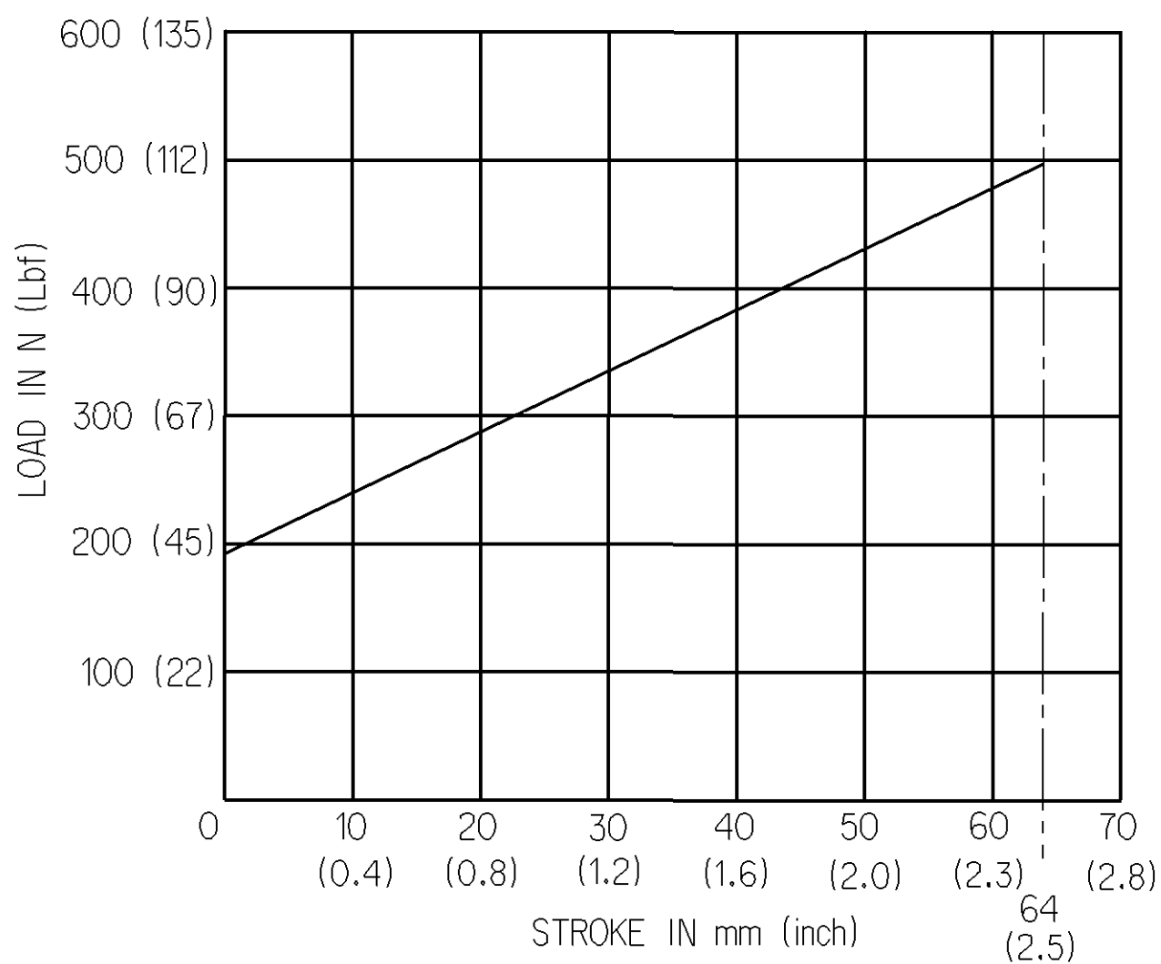
RETURN SPRING CHARACTERISTICS
