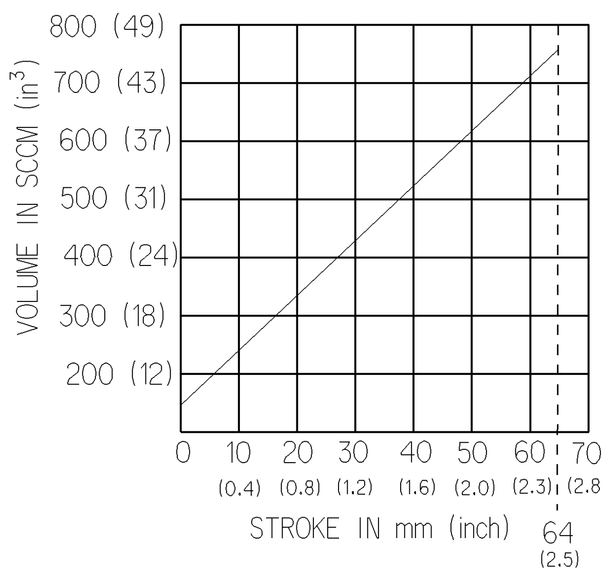
CHAMBER VOLUME vs STROKE
