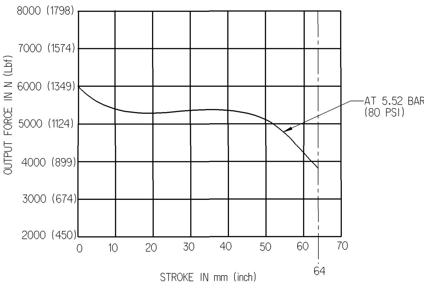
PERFORMANCE CHARACTERISTICS
