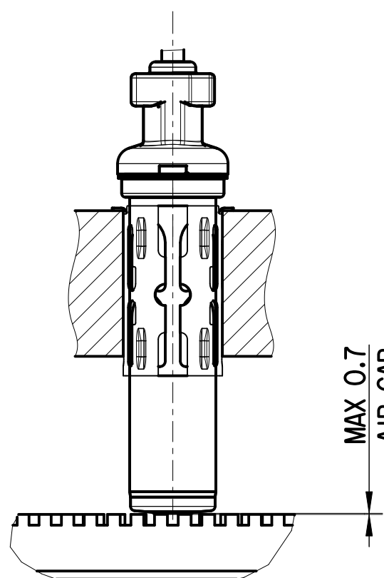
ASSEMBLY VIEW (IN VEHICLE)
