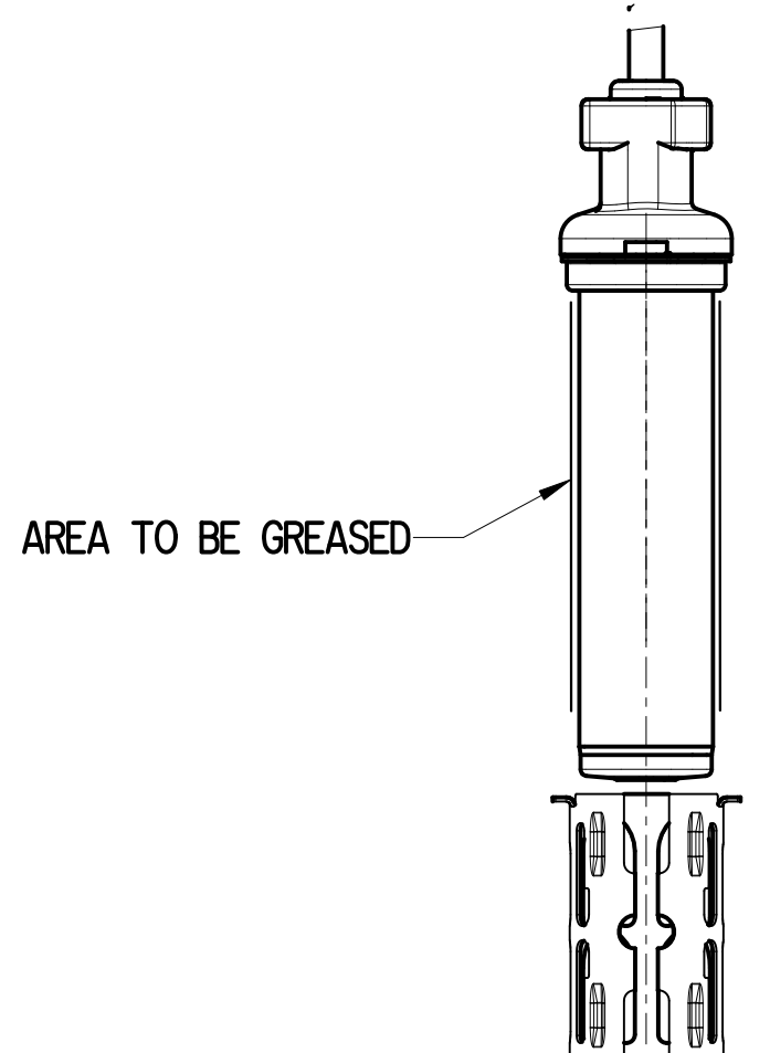
BEFORE ASSEMBLY VIEW
