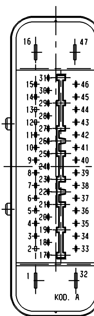
DETAIL X 47 PIN CONNECTOR
