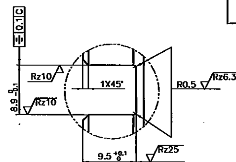
DETAIL E (3:1)
