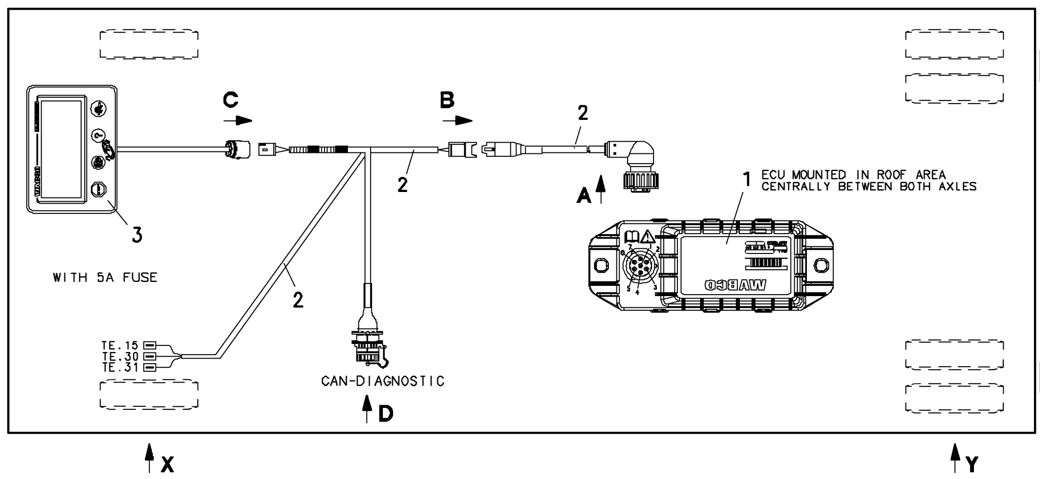
WIRING HARNESS 894 607 390 0
