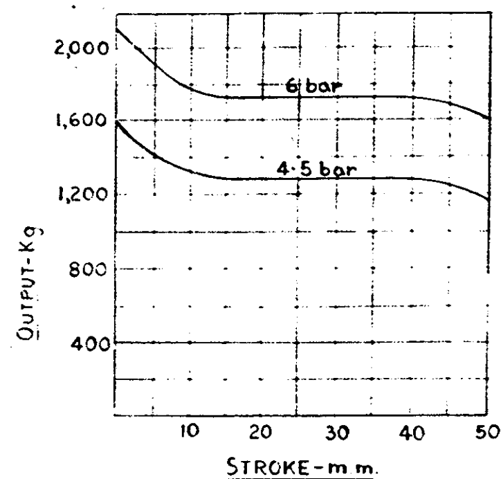
PERFORMANCE CURVE - NOMINAL
