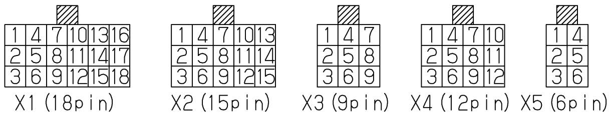
TERMINAL ASSIGNMENT FOR ECU ECU端子配列
